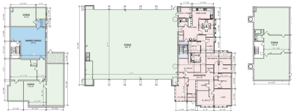
BASEMENT AREA PLAN
